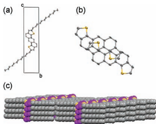
Figure 4. (a) Thermal ellipsoid plot of 5d . View down the a -axis. (b) View down the “stacking axis” of two cofacial molecules of 5d with dodecyl chains omitted. (c) Space-filling diagram of 5d illustrating packing structure. Sulfur atoms are yellow, sp^3 -hybridized carbon atoms are gray, and sp^2 -hybridized carbons atoms are purple.
