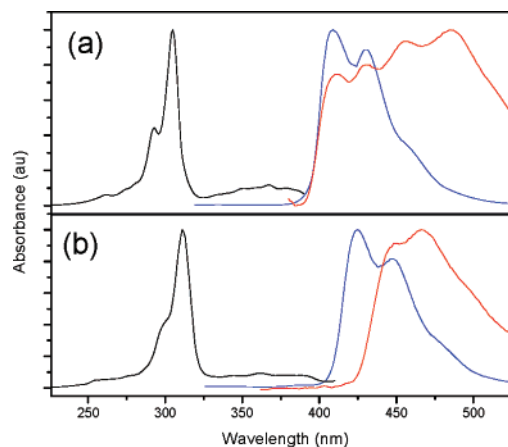
Figure 5. (a) Excitation spectrum of 5a in solution (black). Emission spectrum of 5a in solution (blue) and as a thin film (red). (b) Excitation spectrum of 5d in solution (black). Emission spectrum of 5d in solution (blue) and as a thin film (red).
