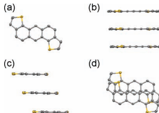
Figure 2. (a) Thermal ellipsoid plot of 5a . (b) View down the short molecular axis of 5a ; the stacking axis is vertical. (c) View down the long molecular axis of 5a ; the stacking axis is vertical. (d) View down the stacking axis of two cofacial molecules of 5a .
