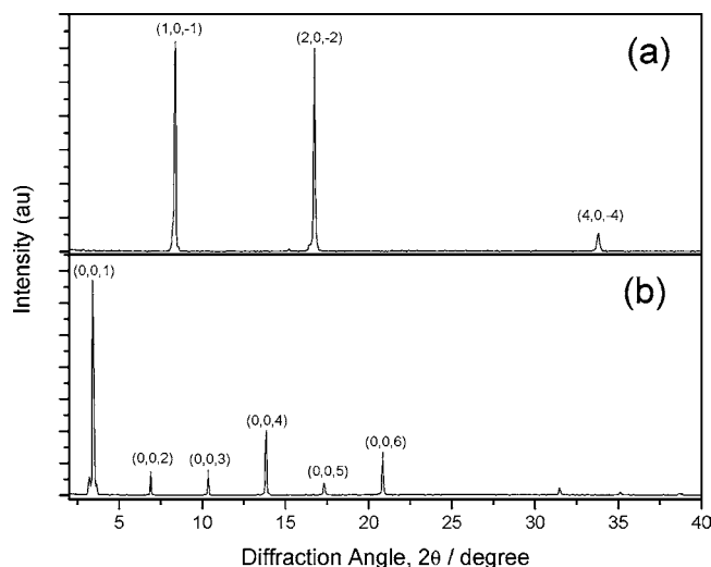
Figure 3. X-ray diffractograms of films of (a) 5a and (b) 5d on glass substrates deposited by vacuum evaporation.
